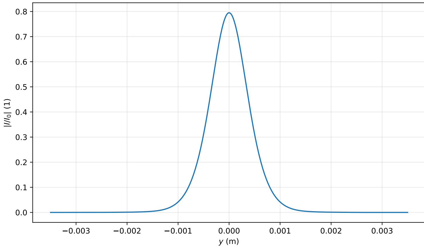
Intensity profile I(x=0, y, z=3.184)/I_0 , P_{in}=0.7P_{cr} , artificial time
